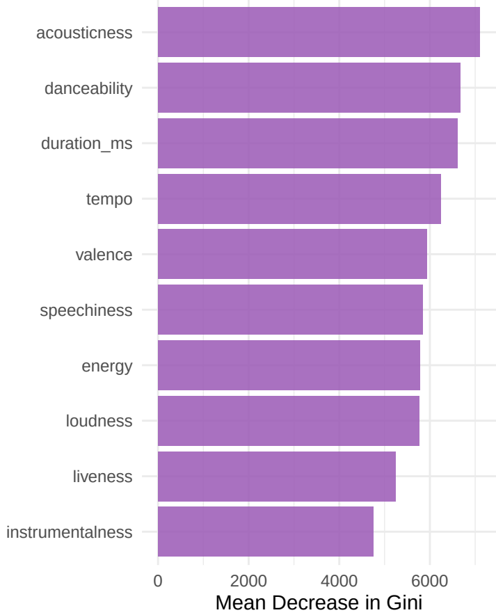
RF Feature Importance (Genre Classification)
