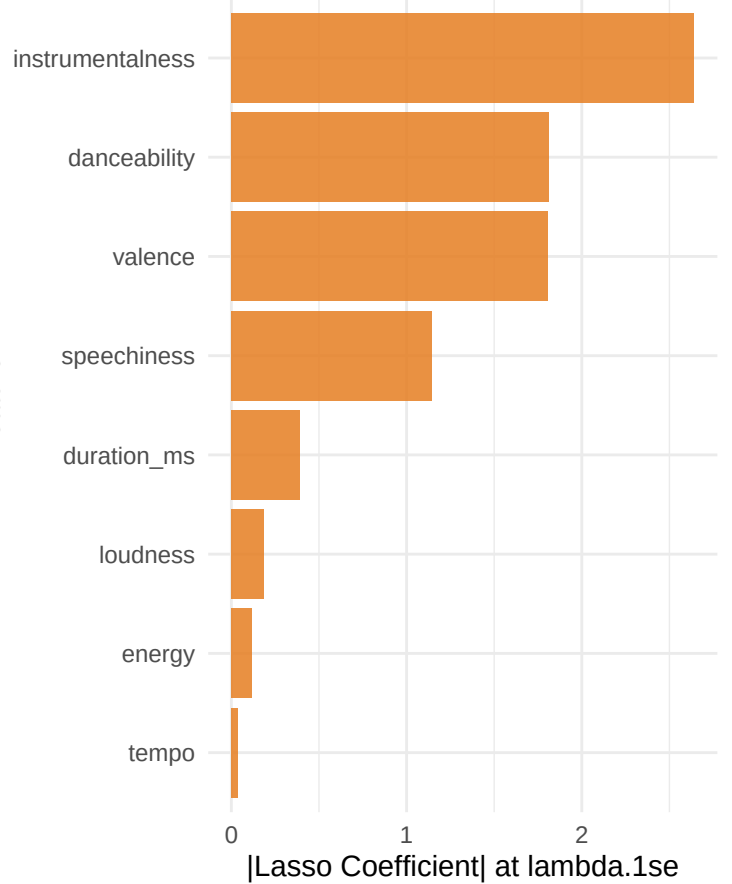
Lasso Feature Importance (Popularity)
