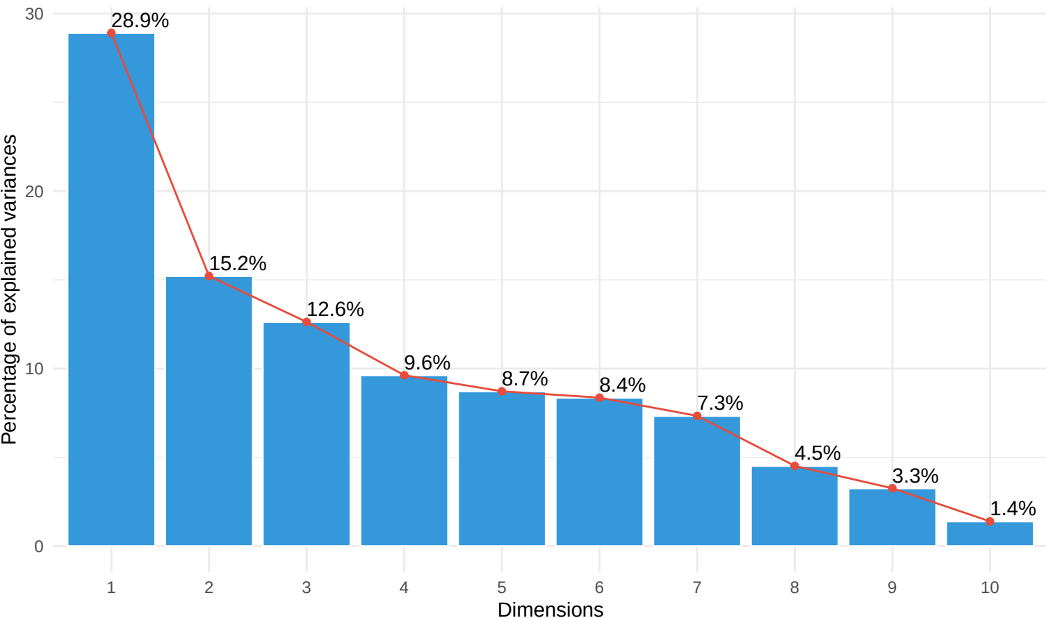
PCA Scree Plot – Variance Explained per Component
