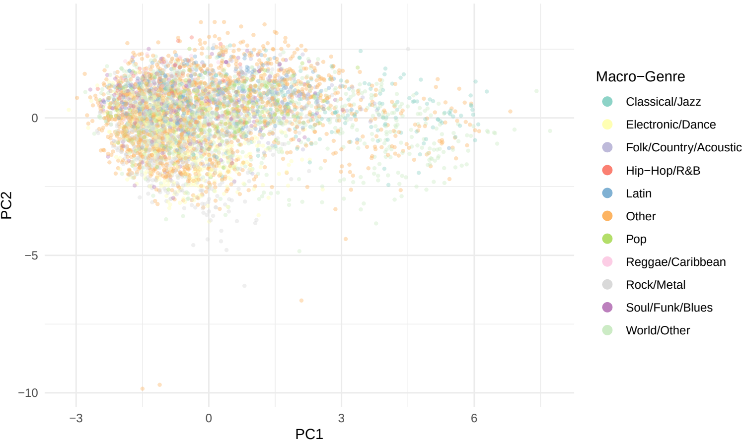
PCA Biplot: PC1 vs PC2 (random sample of 5,000 tracks)
