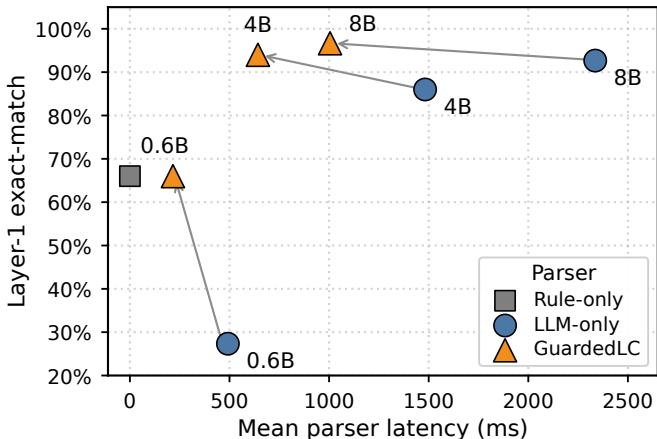
Accuracy-latency trade-off
