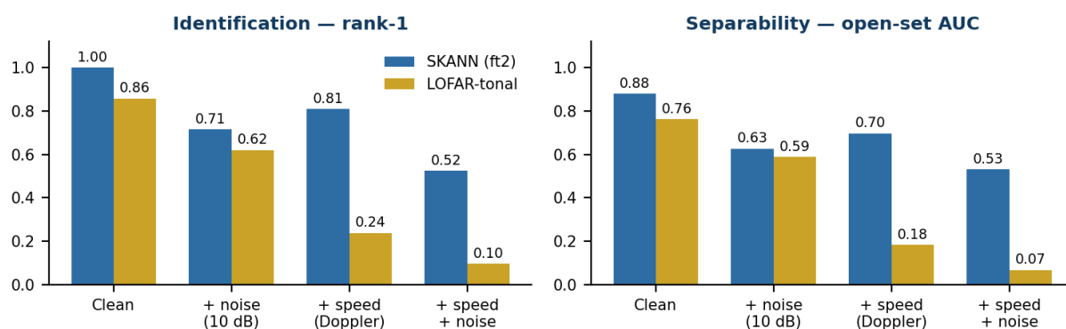
Figure 4 — NODPAC-21 half-split spot-check, four conditions: rank-1 (left) and open-set AUC (right), SKANN ft2 vs LOFAR-tonal. Source: disc5_arcface_8k_allbench_compare_ft2.json.
