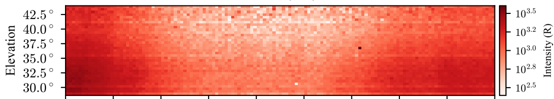
6300 Å (Red)
