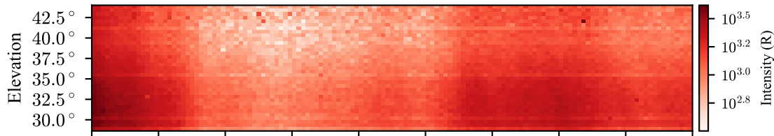
6306 Å (Cloud Indicator)
