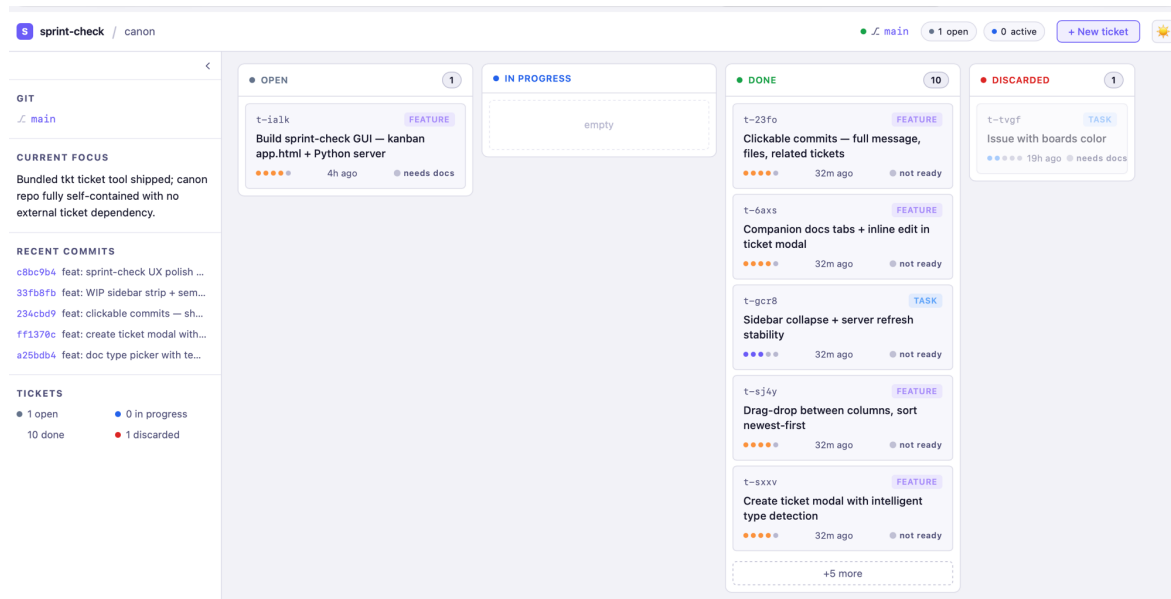
Figure 1: sprint-check board
