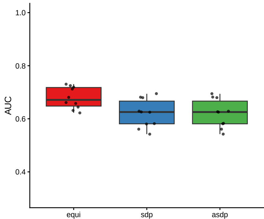
Downstream AUC by knockoff method (best config)
