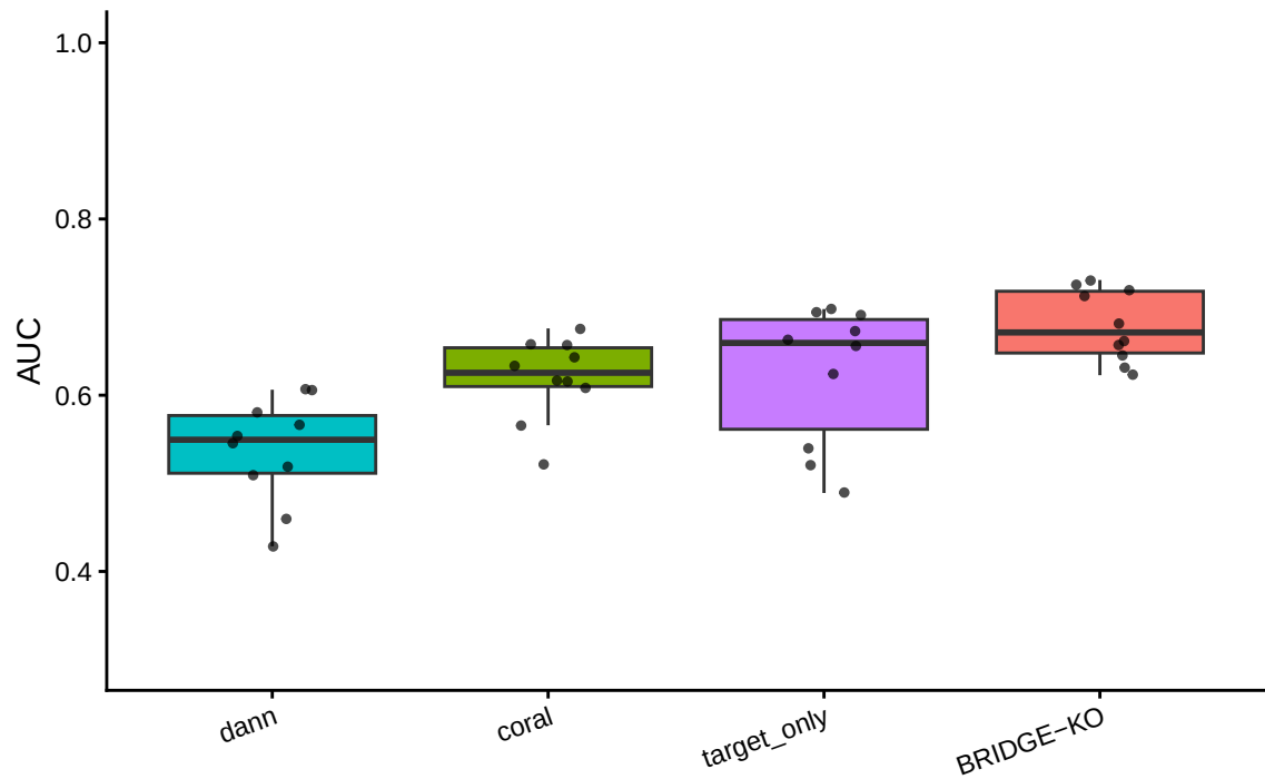
BRIDGE-KO vs baselines (PCA, ComBat-both, top 25%)
