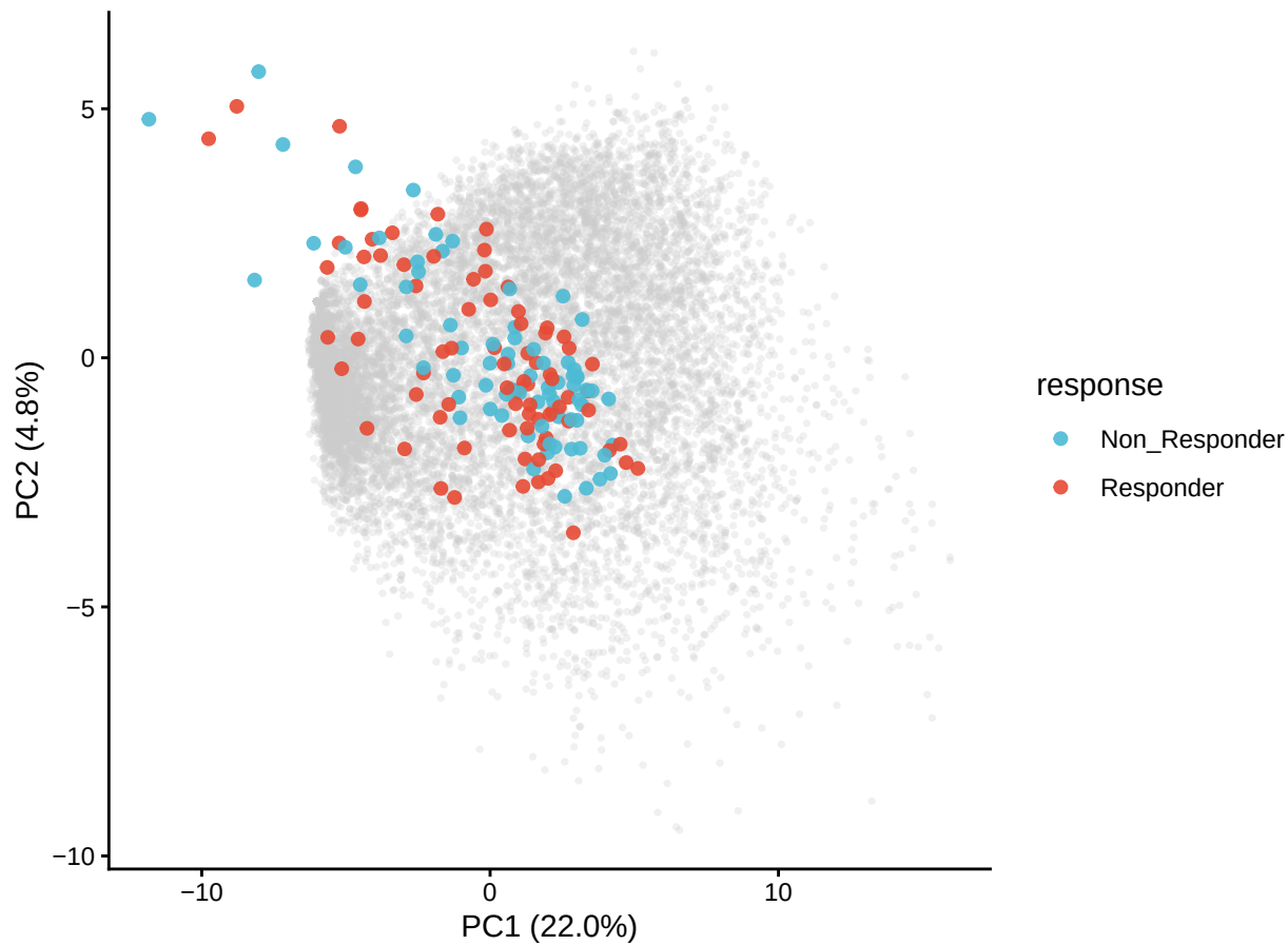
Fig 4E recolored by response (ComBat both)
