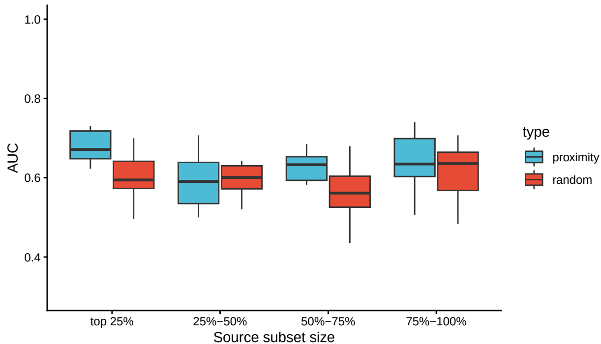
Proximity-ranked vs random source subset (PCA, ComBat-both)
