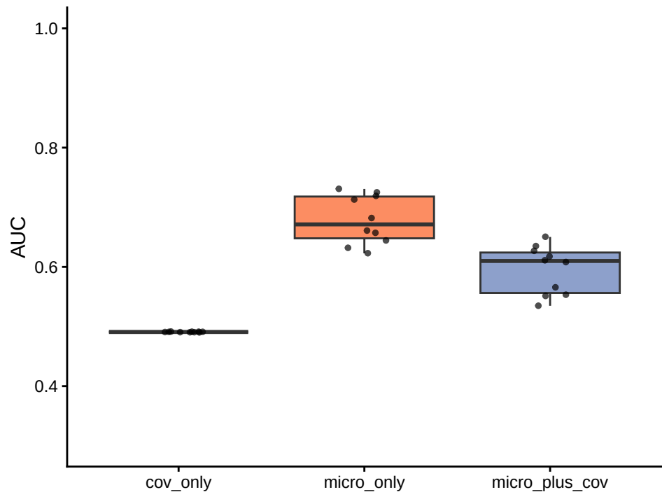
Covariate-augmented prediction (best config)
