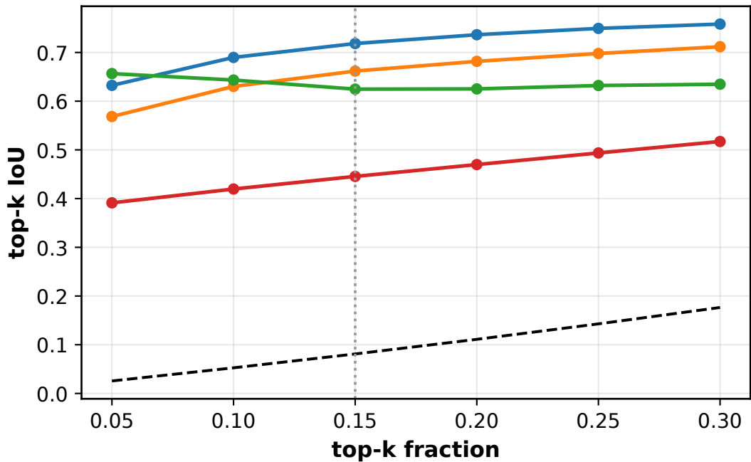
Drift metrics vs top-k threshold (dotted line = reported k)
