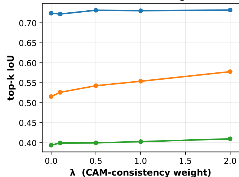
MobileNetV3-Large
