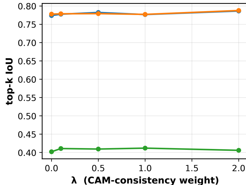
ResNet-50
