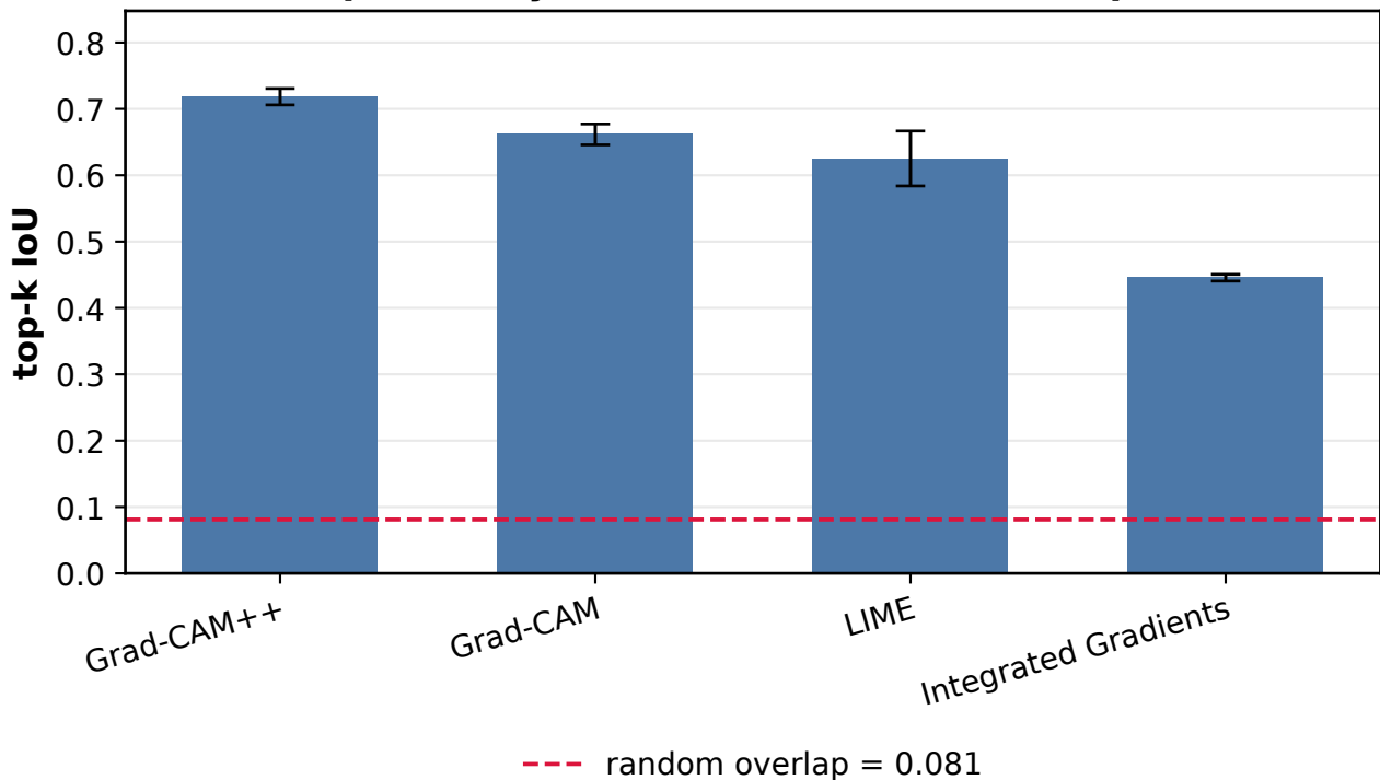
top-k IoU by XAI method (95% bootstrap CI)
