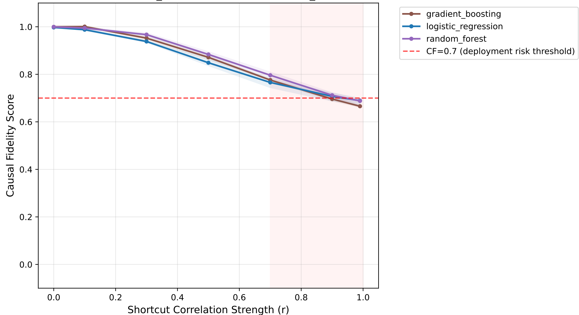
Causal Fidelity vs Shortcut Strength Dataset: adult_income, Shortcut: selection_bias
