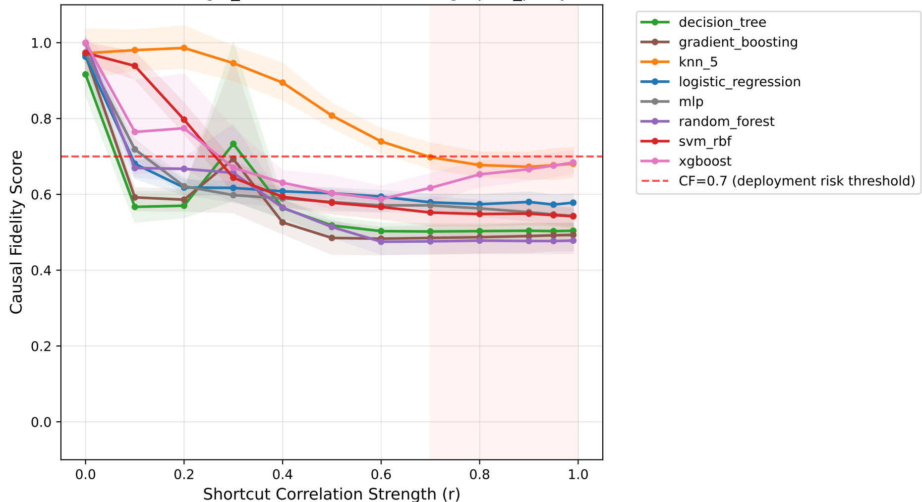
Causal Fidelity vs Shortcut Strength Dataset: bangla_dataset, Shortcut: demographic_proxy
