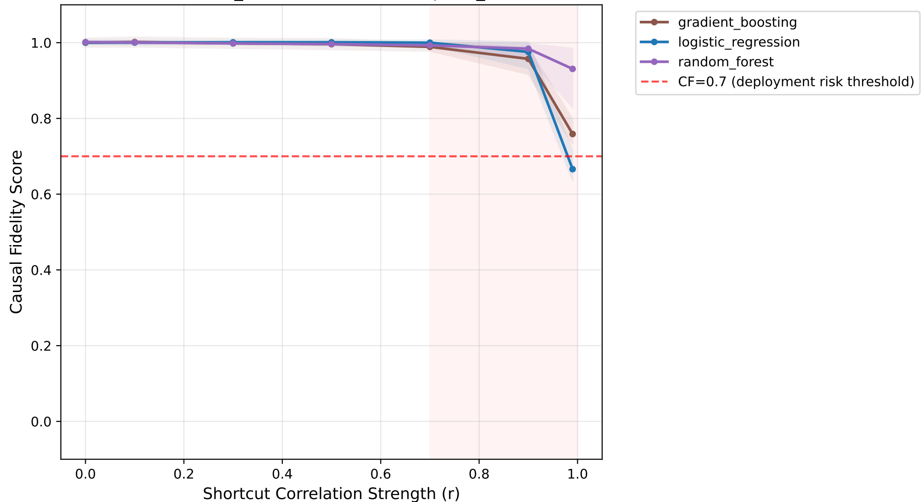
Causal Fidelity vs Shortcut Strength Dataset: credit_default, Shortcut: temporal_shortcut
