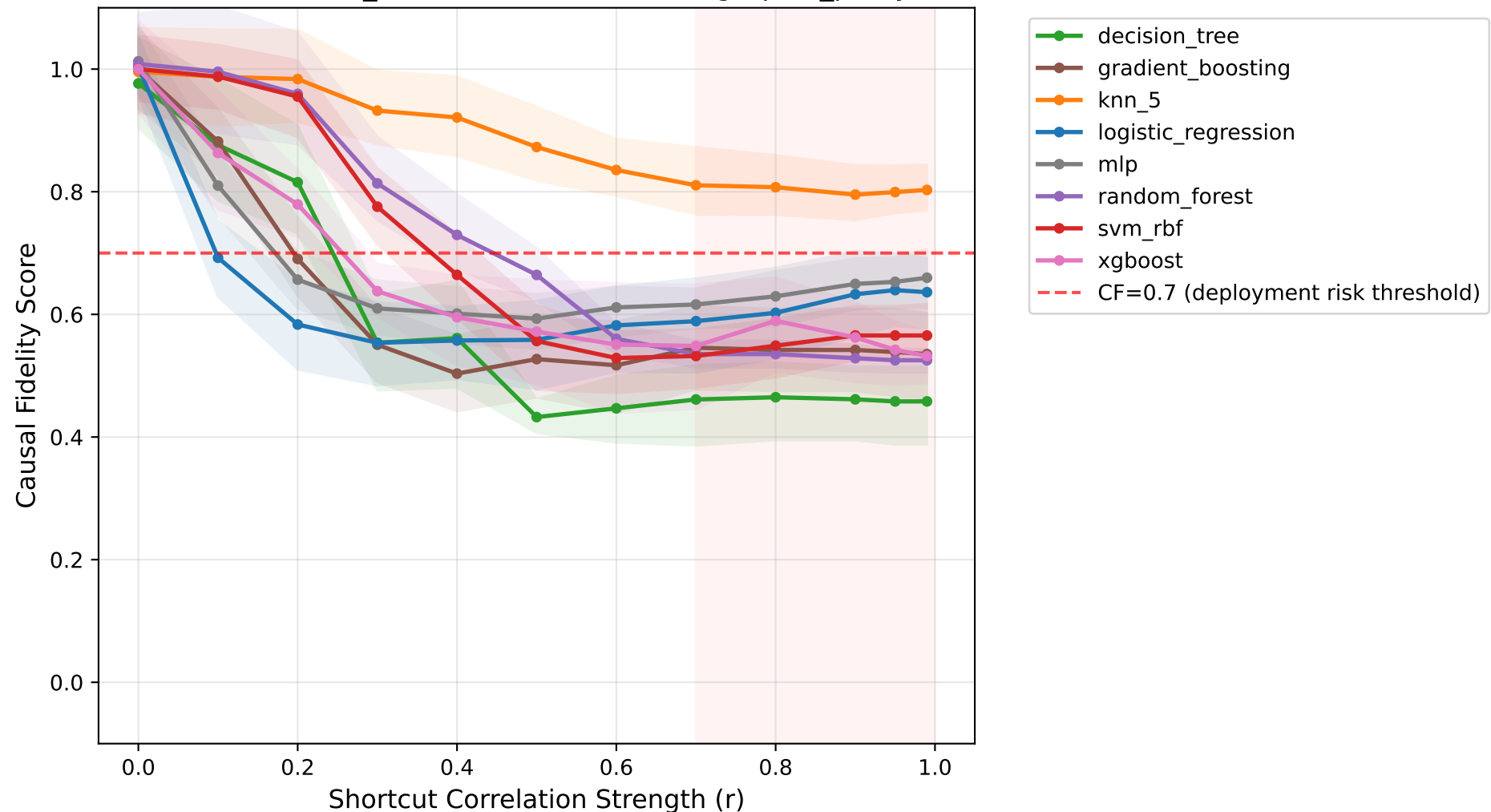
Causal Fidelity vs Shortcut Strength Dataset: heart_disease, Shortcut: demographic_proxy
