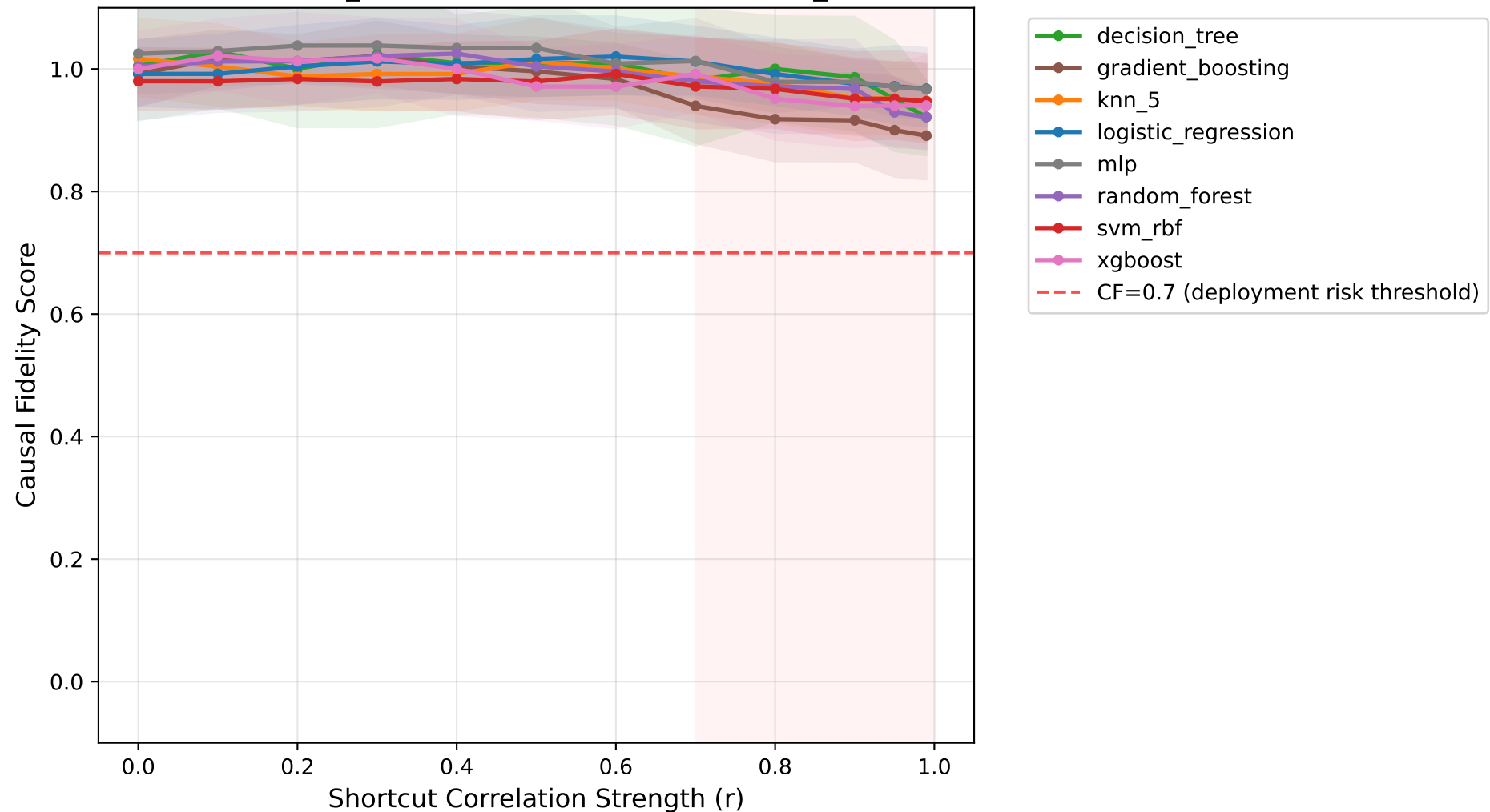
Causal Fidelity vs Shortcut Strength Dataset: heart_disease, Shortcut: measurement_artifact
