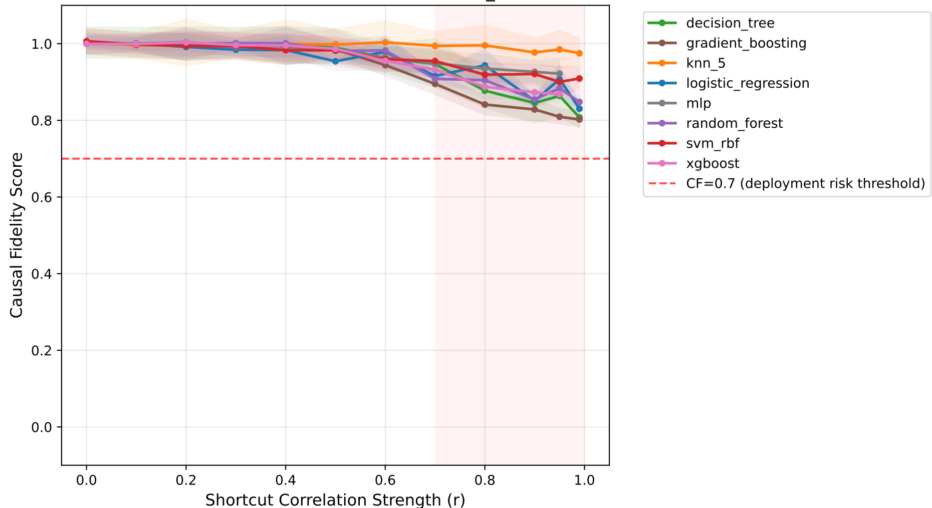
Causal Fidelity vs Shortcut Strength Dataset: madelon, Shortcut: measurement_artifact
