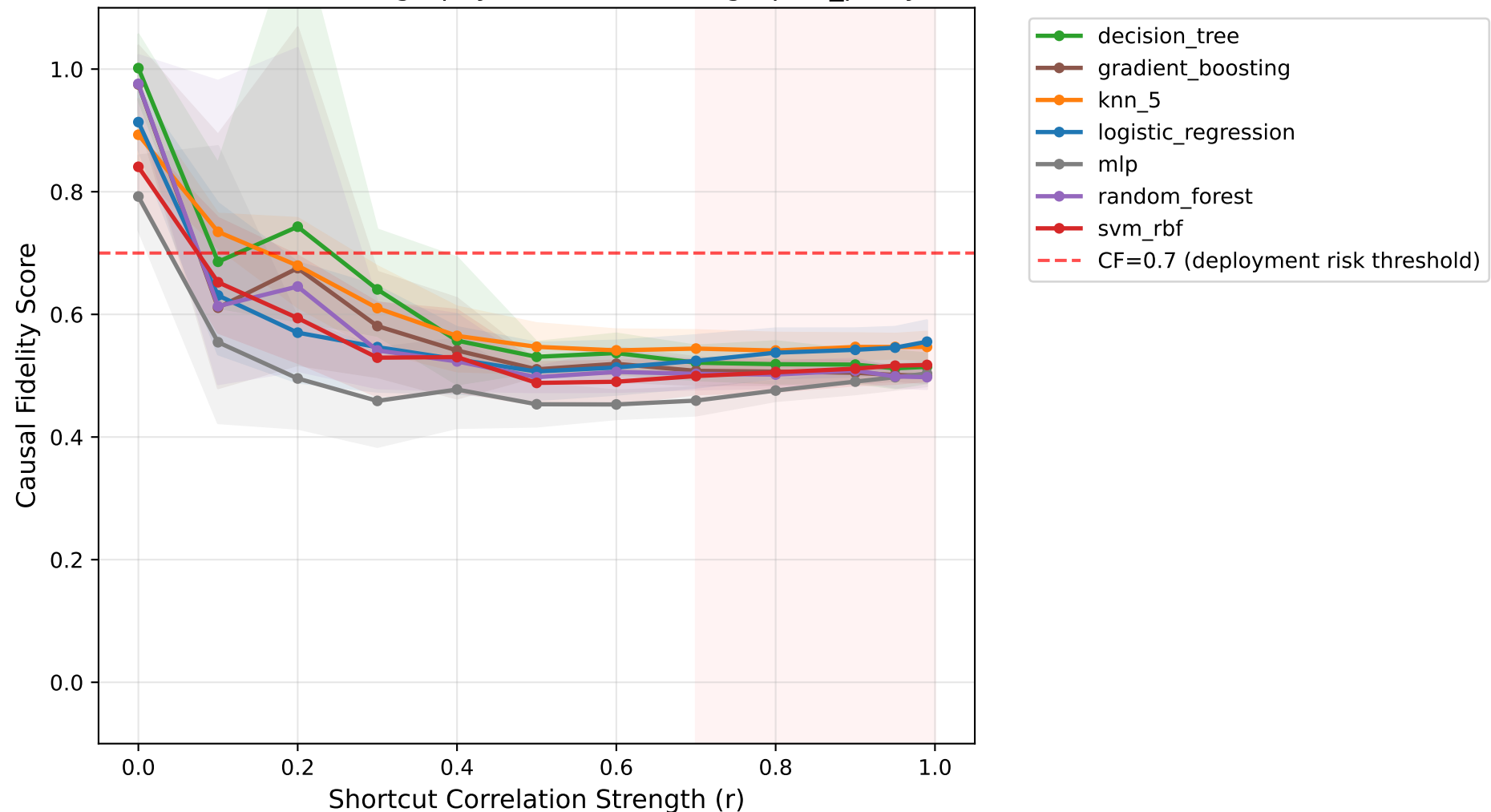
Causal Fidelity vs Shortcut Strength Dataset: mammography, Shortcut: demographic_proxy
