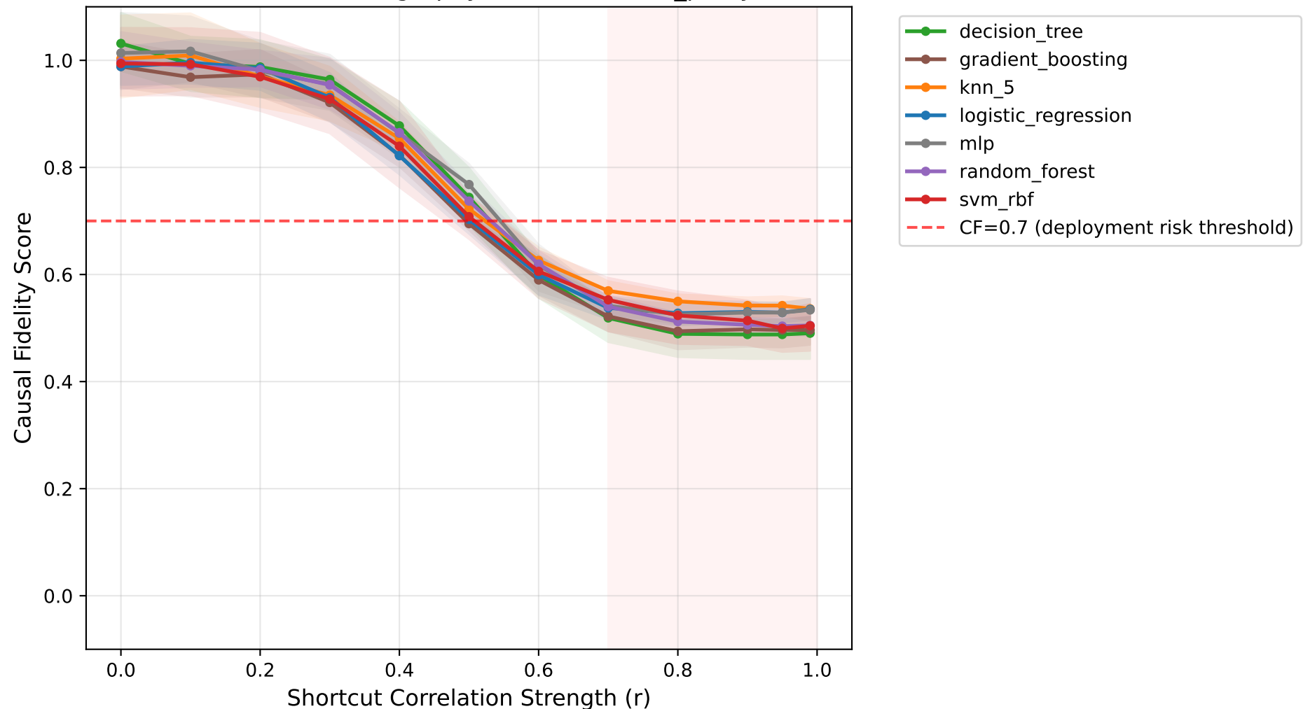
Causal Fidelity vs Shortcut Strength Dataset: mammography, Shortcut: label_proxy
