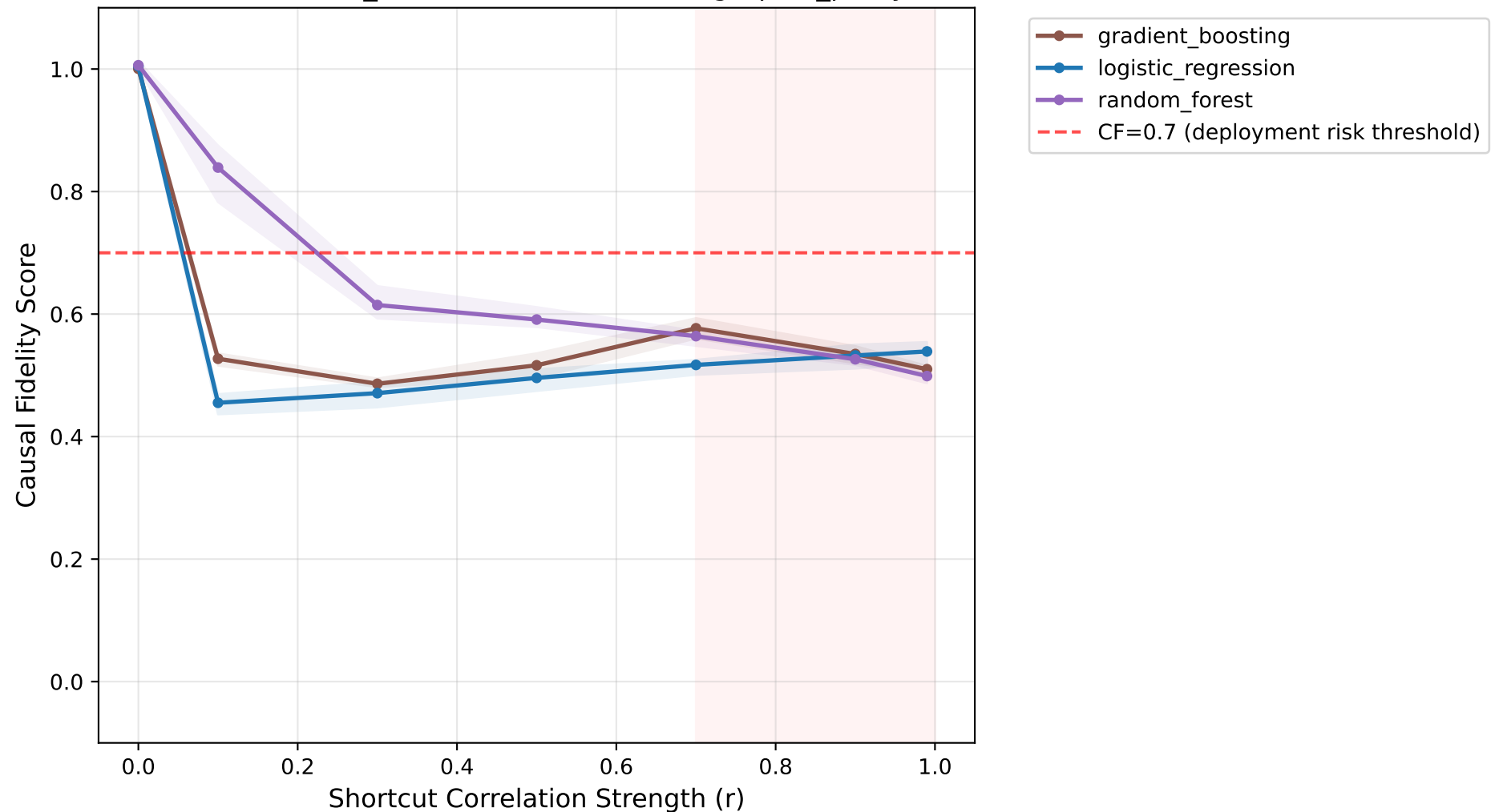
Causal Fidelity vs Shortcut Strength Dataset: adult_income, Shortcut: demographic_proxy
