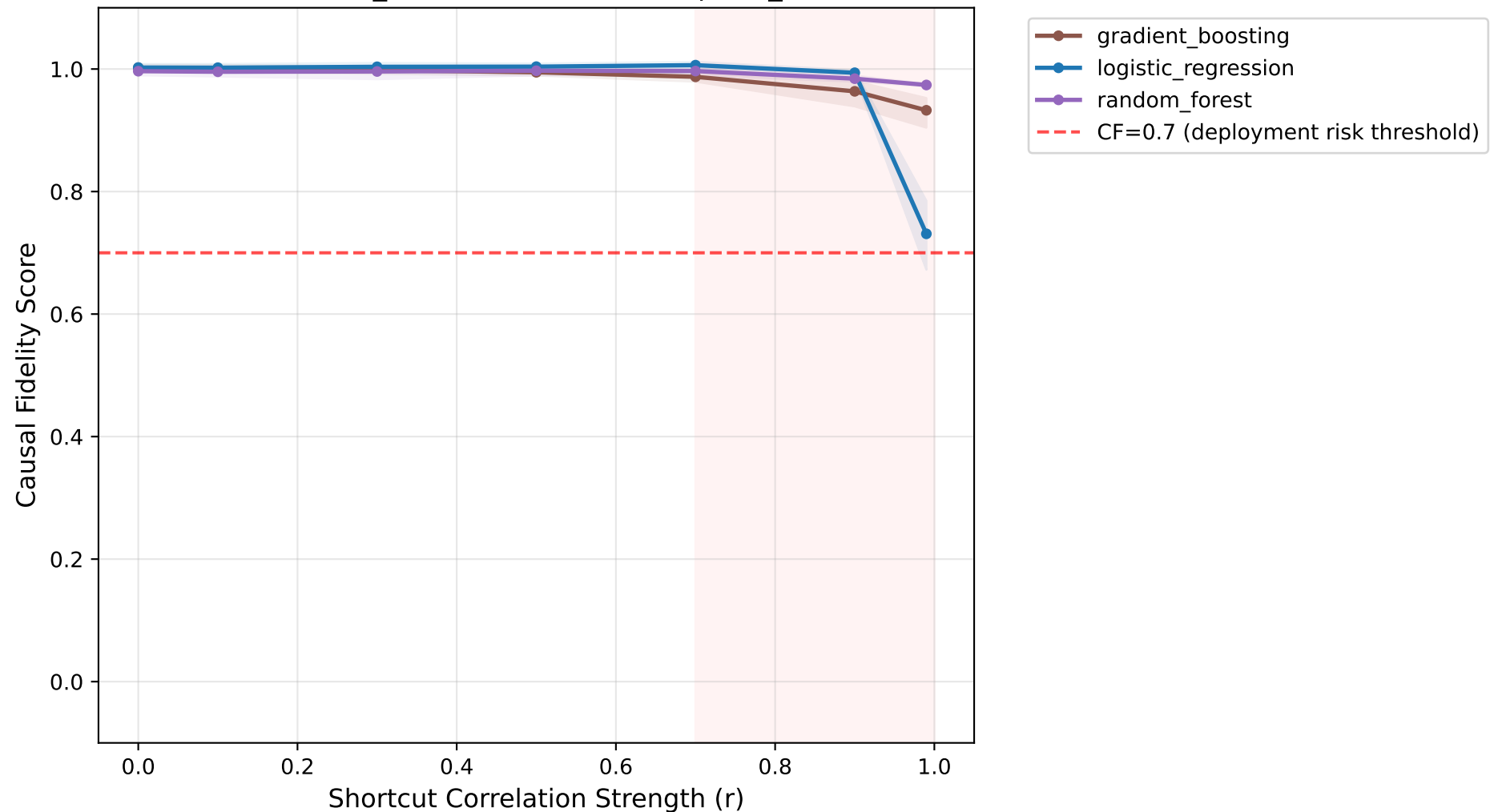
Causal Fidelity vs Shortcut Strength Dataset: adult_income, Shortcut: temporal_shortcut
