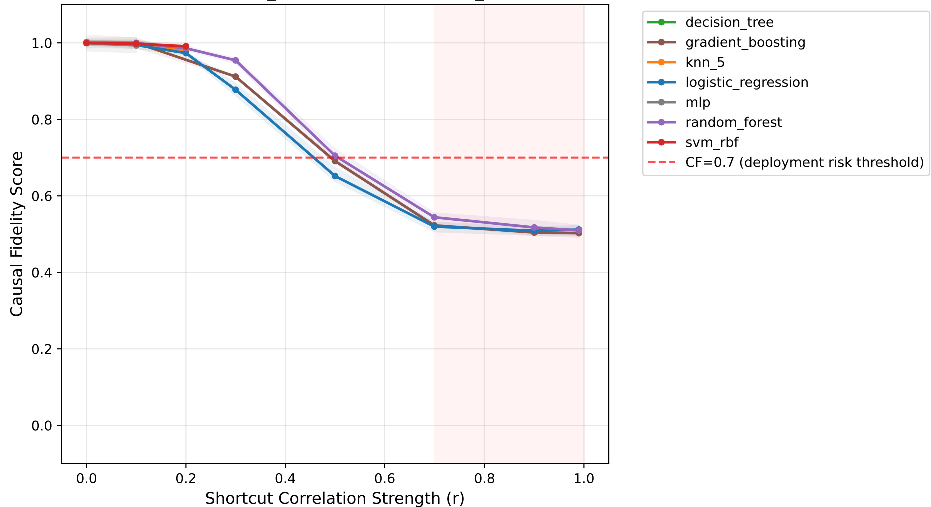
Causal Fidelity vs Shortcut Strength Dataset: credit_default, Shortcut: label_proxy
