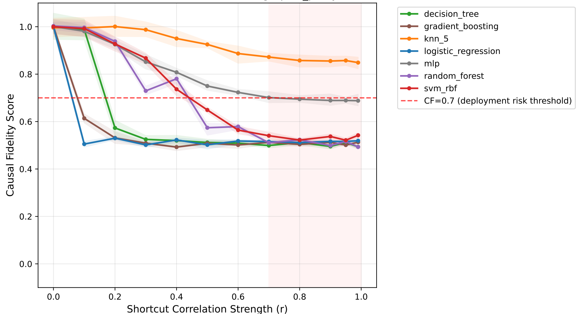
Causal Fidelity vs Shortcut Strength Dataset: madelon, Shortcut: demographic_proxy
