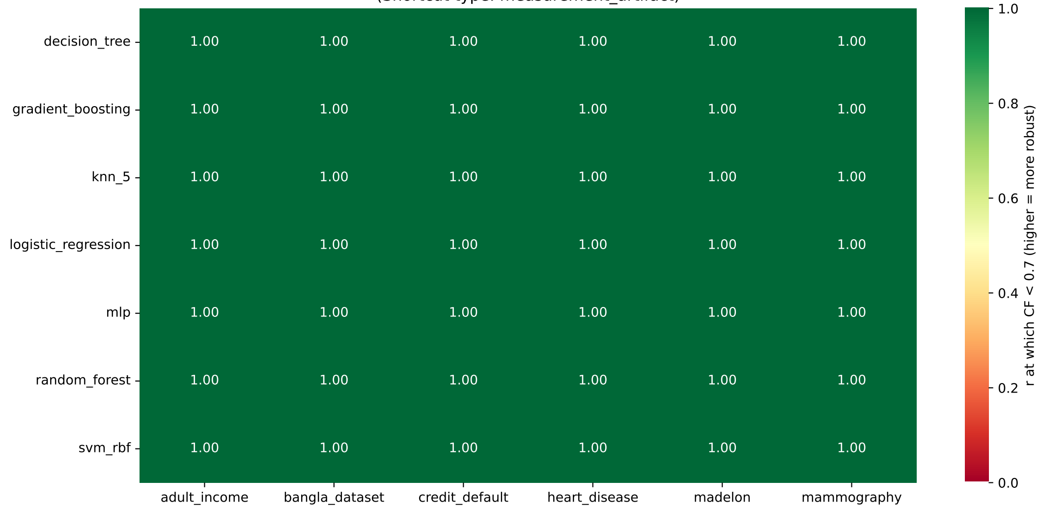
Phase Transition Heatmap: Shortcut Tolerance by Model and Dataset (Shortcut type: measurement_artifact)
