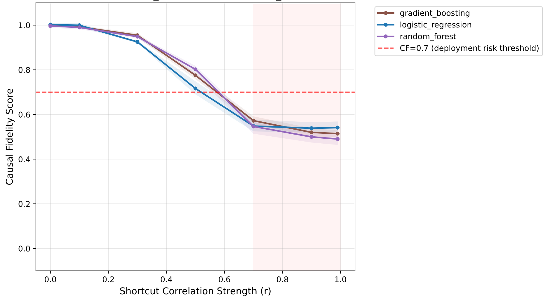
Causal Fidelity vs Shortcut Strength Dataset: adult_income, Shortcut: label_proxy
