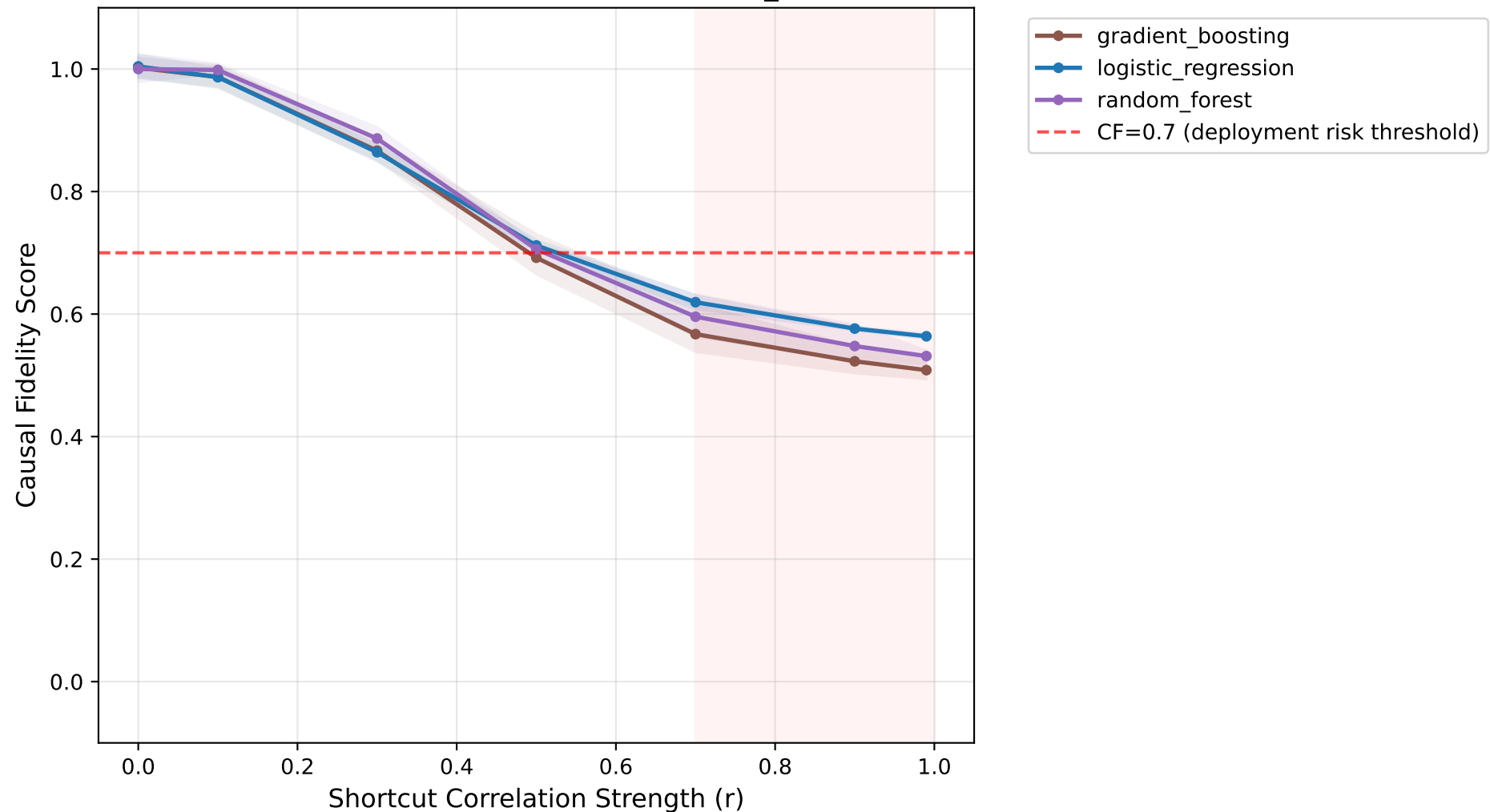
Causal Fidelity vs Shortcut Strength Dataset: madelon, Shortcut: selection_bias
