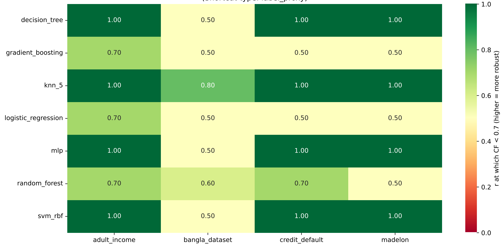
Phase Transition Heatmap: Shortcut Tolerance by Model and Dataset (Shortcut type: label_proxy)
