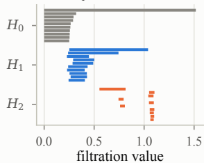
persistence of z
