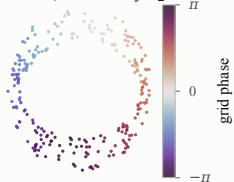
PC3-PC4, coloured by \theta_2
