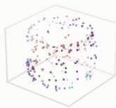
canonical latent (PC1-3)
