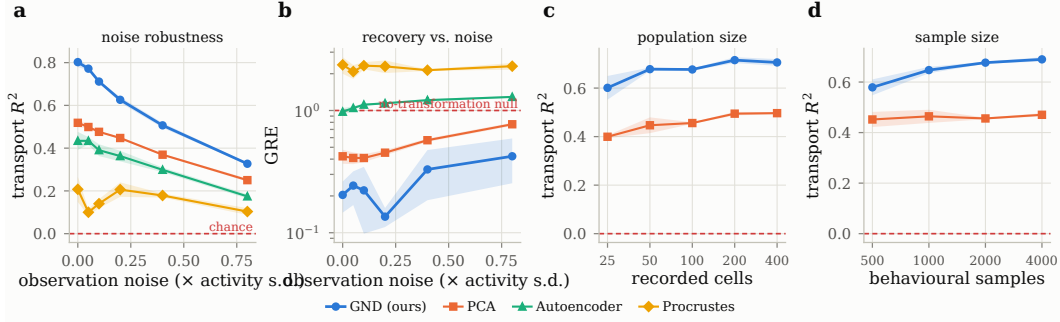
Figure 8: Robustness and scaling. (a,b) Observation noise. (c) Number of recorded cells. (d) Number of behavioural samples.
