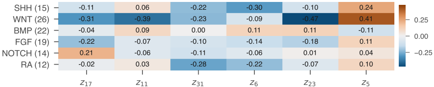
Pearson correlation between latent channel and morphogen-pathway score
