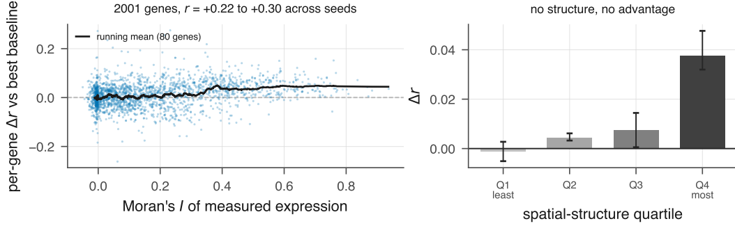
Figure 2: The advantage appears only where there is spatial structure to exploit. Left: every gene, held-out per-gene Pearson r against the strongest baseline, versus the Moran's I of the measured signal; the running mean rises from zero to roughly 0.048. Right: quartile means, bars spanning the range across 3 seeds. The least-structured quartile straddles zero. This is a sharper test than any aggregate number because the mechanism predicts where the model should stop winning, and it does.
