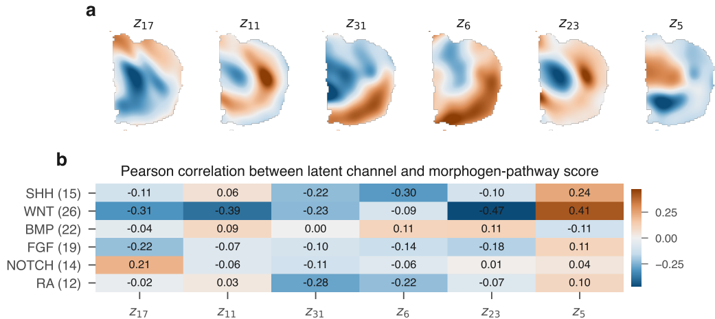
Figure 6: Latent channels of the relaxed field (a) and their correlation with canonical morphogen-pathway scores (b). Section 5.6 shows these correlations do not survive a causal split-half test.
