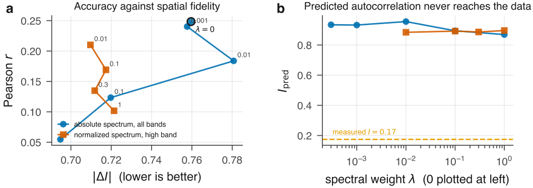
Figure 5: Spectral matching. (a) The trade-off: up and to the left is better. Points are labeled by weight \lambda ; \lambda = 0 is the model used everywhere else. (b) Predicted global autocorrelation against \lambda . No weight of either form brings I_{\text{pred}} near the measured value.
