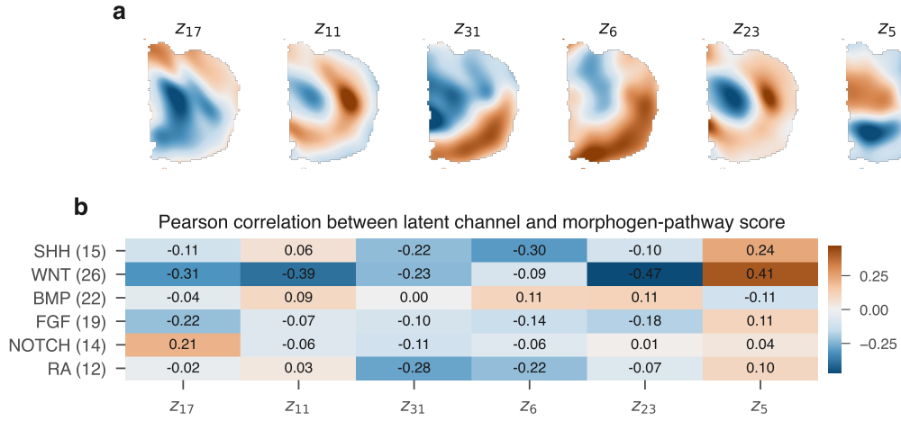
Figure 5: Latent channels of the relaxed field (a) and their correlation with canonical morphogen-pathway scores (b). Section 5.6 shows these correlations do not survive a causal split-half test.
