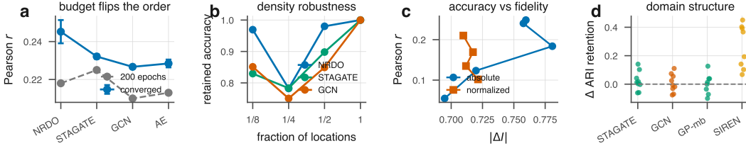
Figure 3: Four checks on the benchmark. (a) The reduced training budget is not neutral: on the section whose ordering depends on it, training to convergence reverses the ordering in our favor. (b) Retained accuracy under uniform subsampling; a model defined on a field rather than a lattice should survive this, and it is the one corruption axis where NRDO clearly leads. (c) Spectral matching trades accuracy for spatial fidelity along both forms tested and bounds rather than removes the over-smoothing. (d) Per-section difference in ARI retention against each baseline: NRDO separates from the implicit neural field and not from the graph models.
