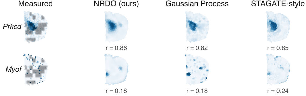
Figure 4: Predicted expression at held-out locations. Grey marks the contiguous blocks hidden from every encoder. Genes are chosen to span the performance range rather than to favor any model — the top row is a well-reconstructed gene, the bottom row one near the lower quartile — and the per-gene r printed beneath each map is for that gene alone, not the benchmark mean. The failure mode the paper reports is visible directly: our predictions are smoother than the measurement, which costs us Moran’s I even where correlation is comparable.
