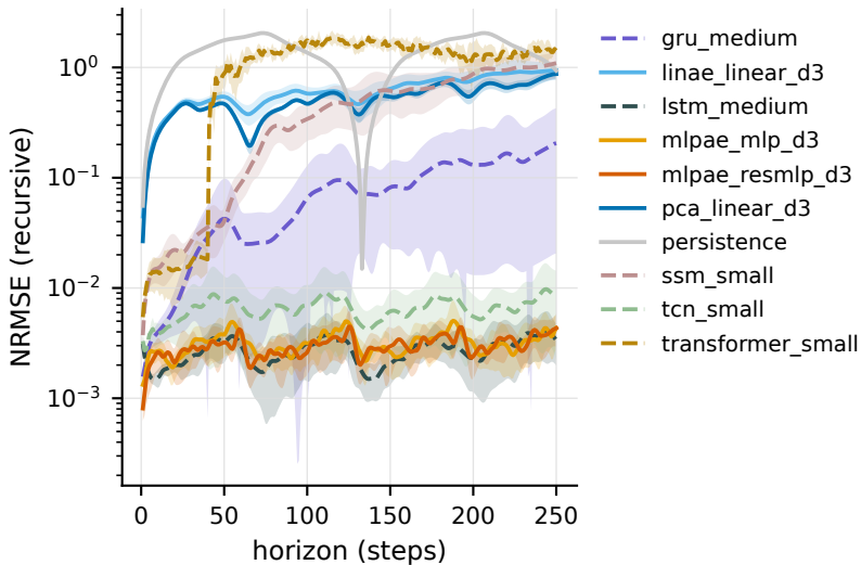
vanderpol: NRMSE vs horizon (test, mean \pm std, n=5 seeds)
