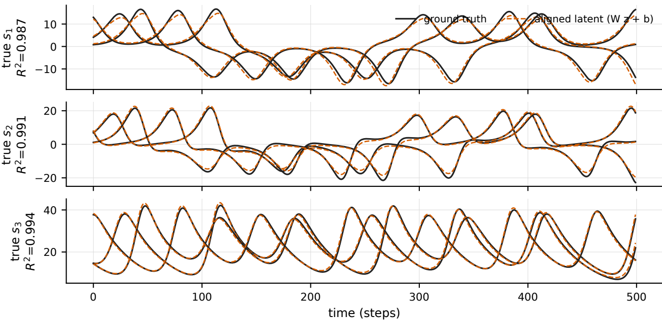
Latent vs ground truth — EXP-0353 — linear alignment R^2=0.991 ( d=3 \rightarrow 3 )
