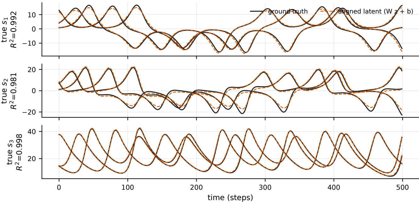
Latent vs ground truth — EXP-0044 — linear alignment R^2=0.990 ( d=3 \rightarrow 3 )
