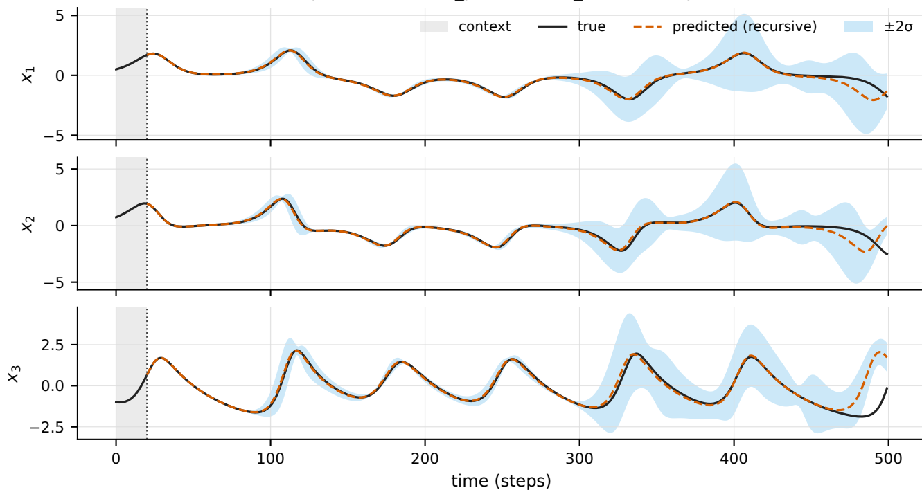
Recursive rollout — EXP-0044 (test split) [ \pm 2\sigma : initial_perturbation_ensemble(eps=0.01)]: context=20, horizon=480
