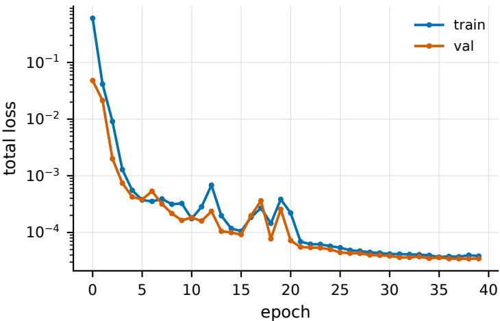
Training — EXP-0044 (n_epochs=40)
