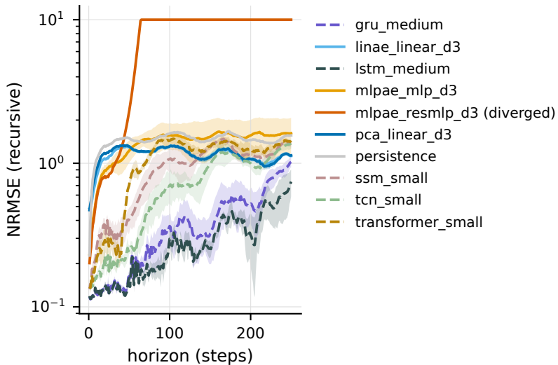
lorenz63_highdim: NRMSE vs horizon (test, mean \pm std, n=5 seeds)
