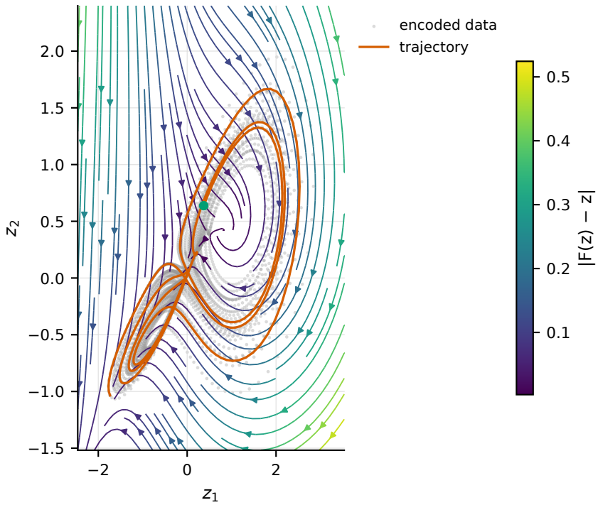
Latent map — EXP-0353: F(z) - z (other 1 dims at mean)
