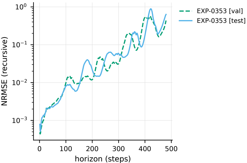
Rollout NRMSE vs horizon — EXP-0353
