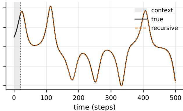
recursive (H=480)
