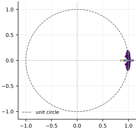
Latent Jacobian eigenvalues — EXP-0044 \max|\lambda|=1.093 ; 290/768 outside unit circle
